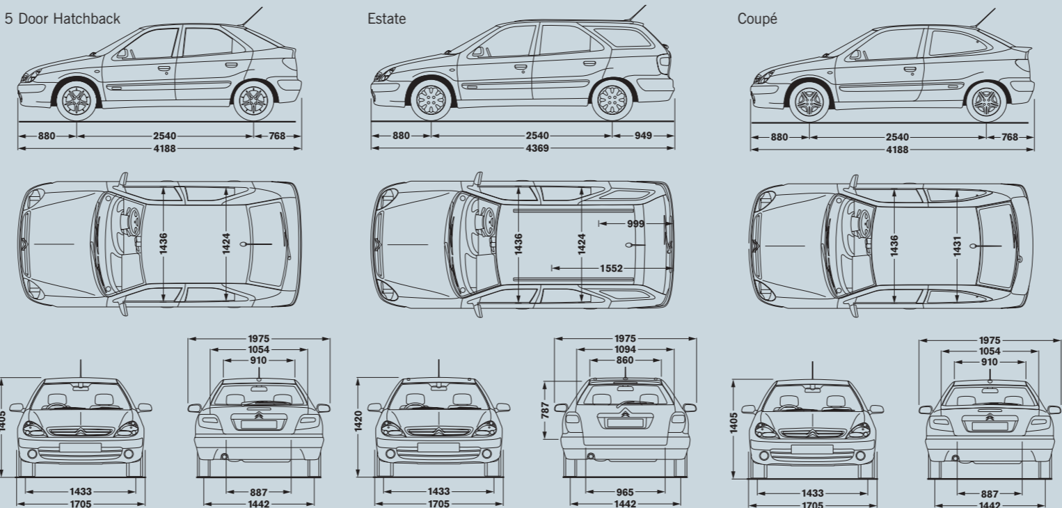
All measurements in millimetres
